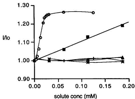
Figure 1. Change in fluorescence emission ( \lambda_{ex} 389 nm, \lambda_{em} 423 nm) for PA-2 upon titration with: \circ 5'-UTP 4- ; \blacksquare fructose; \blacktriangle 2'-deoxy-5'-UTP 4- , + 5'-UMP 2- , and \times 5'-UDP 3- , in phosphate buffer solution (pH 7.3, 15 mM), T = 298 K.
